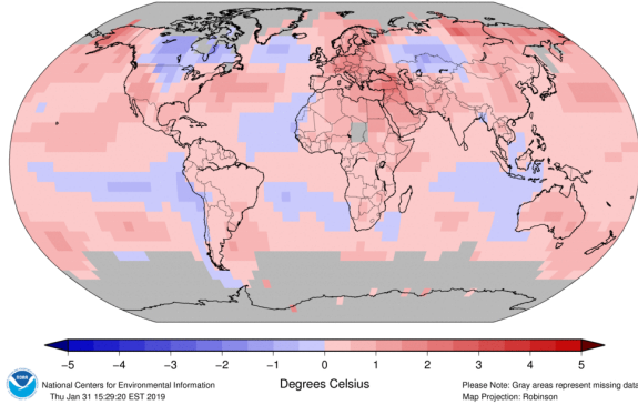
Land & Ocean Temperature Departure from Average Jan–Dec 2018 (with respect to a 1981–2010 base period) Data Source: GHCN–M version 3.3.0 & ERSST version 4.0.0
